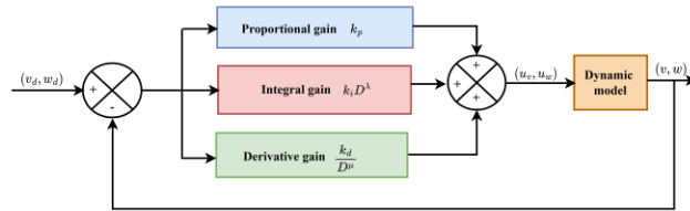
Figure 4 Dynamic controller of DDMR based on FOPID.
