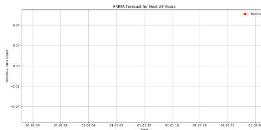
Figure 6: Forecasts from ARIMA (flat lined at 0)
