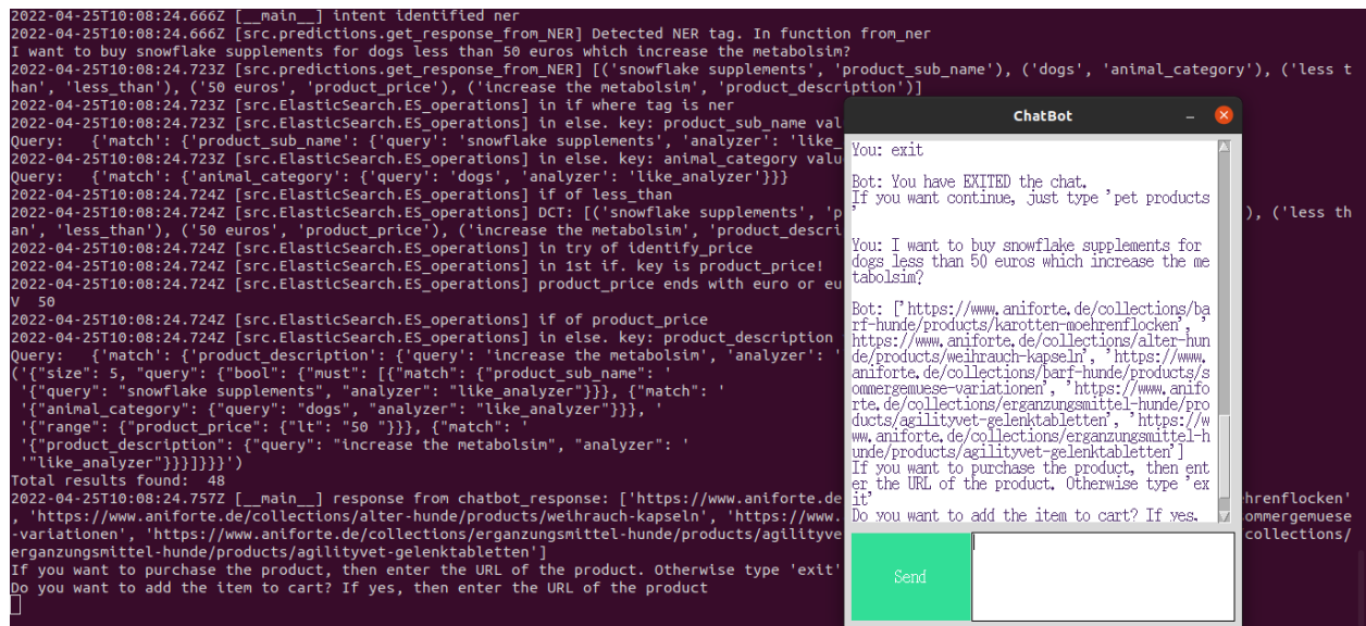
Figure 7: Find the products directly using NER concept
