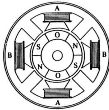
Sketch-3 Motor with Two Phases of BLDC Current
