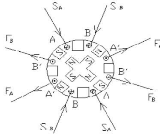
Sketch-7. A motor with no brushes
