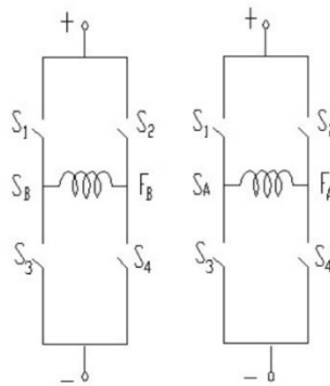
Sketch-8. the transition of the stator between process A and process B
