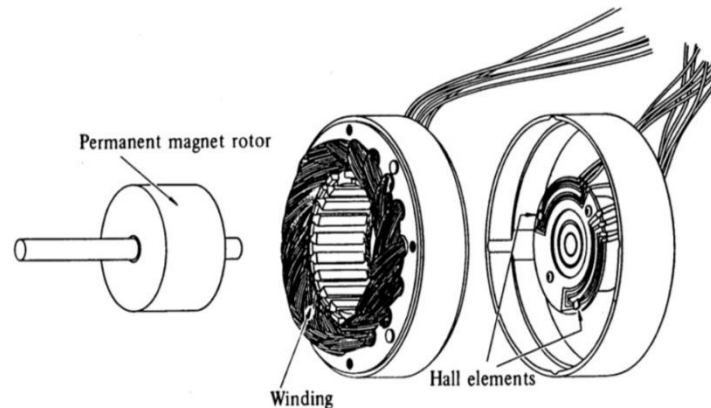
Sketch-1. Internal Organization of a Brushless Direct Current Motor
