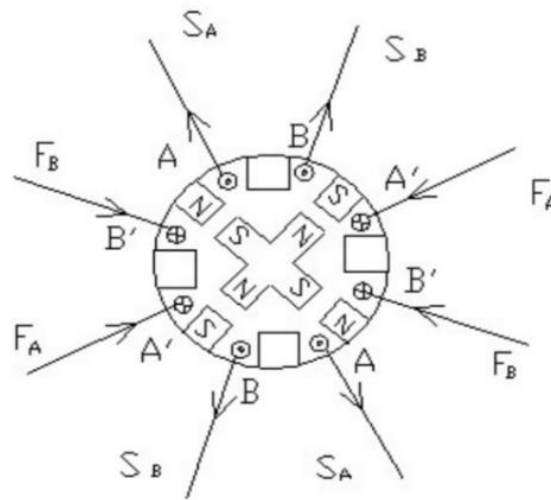
Sketch-5. A brushless direct current motor
