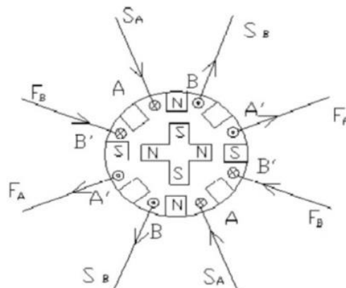
Sketch-6. A motor with no brushes
