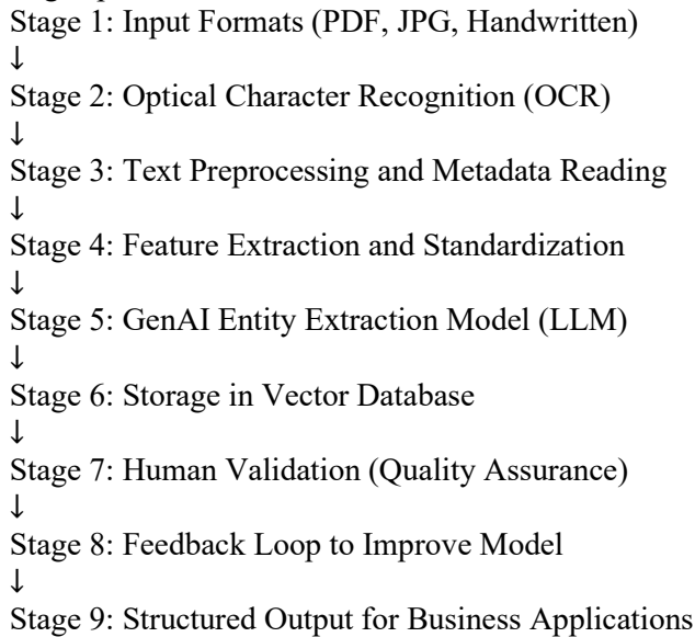
Figure 1: End-to-end architecture for centralized invoice processing combining OCR and LLM technologies
