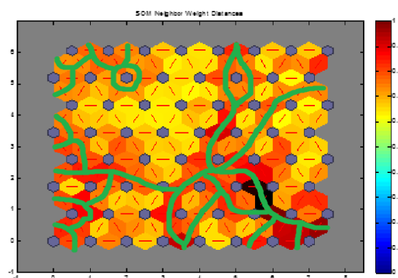
Figure 5: Distances between neurons as measured in Euclidean space
