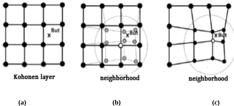
Figure 3: Example of adopting the SOM technique: (a) lag phase, (b) phase k situation, and (c) phase k+1 state.
